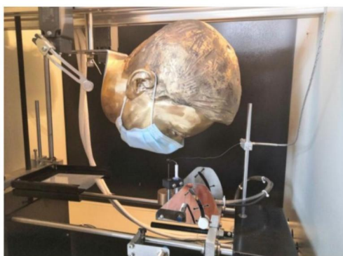
Flame-Resistance Tester
